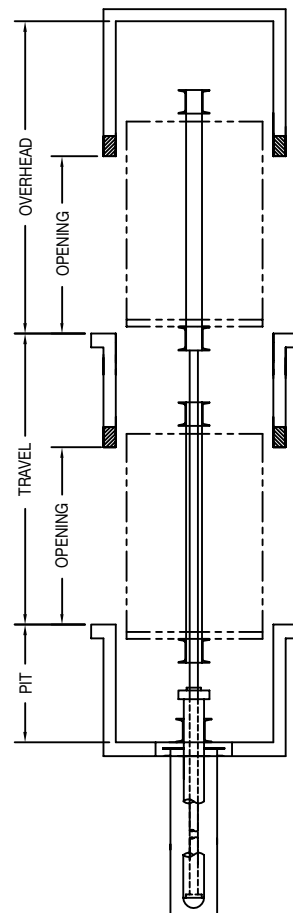
BOREHOLE
